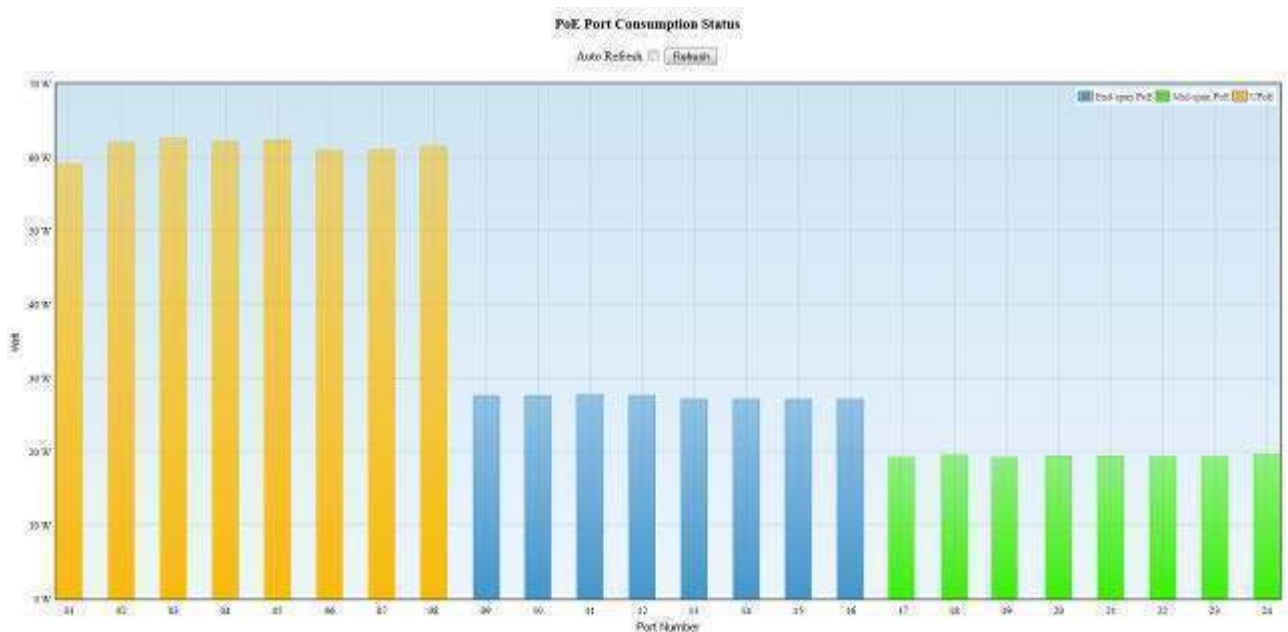
Figure 4-5-6: PoE Status Screenshot
