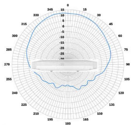
CW9176D 5 GHz Radio Slot 1
