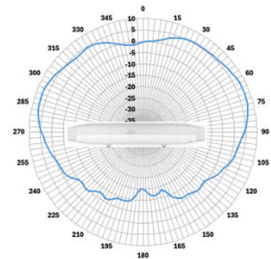
CW9176I 5 GHz Radio Slot 2
