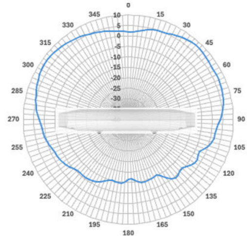
CW9176I 5 GHz Radio Slot 2
