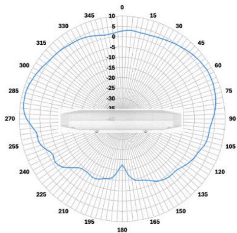
CW9176I 5 GHz Radio
