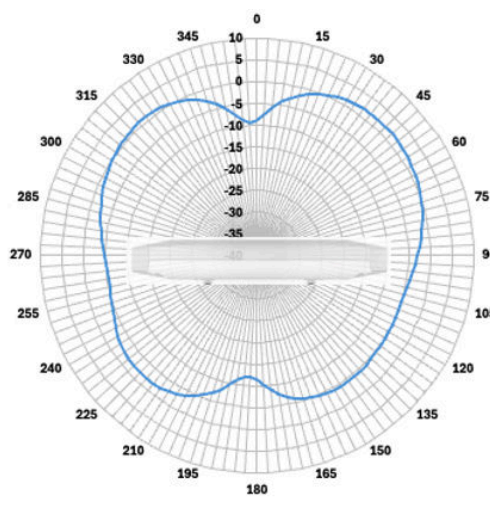
CW9176I GNSS Radio
