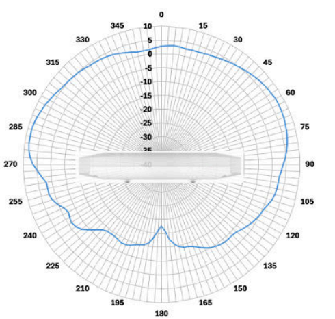
CW9176D 5 GHz Radio
