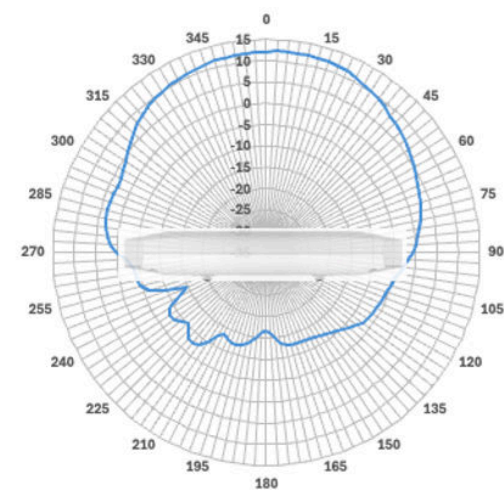
CW9176D 2.4 GHz Radio
