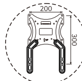
VESA 200x300
